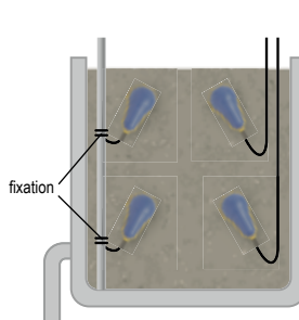
MULTI-LEVEL SWITCHING
