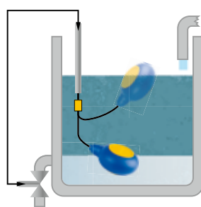
EMPTYING CONTROL
