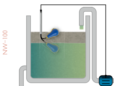
FILLING CONTROL
