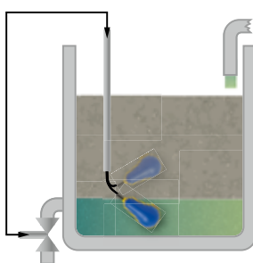
EMPTYING CONTROL
