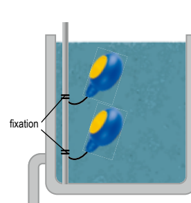
MULTI-LEVEL SWITCHING
