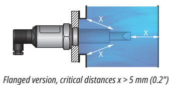
Flanged version, critical distances x > 5 mm (0.2")
