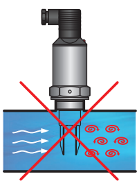
For pipe mounting, the prongs must be parallel to the direction of flow
