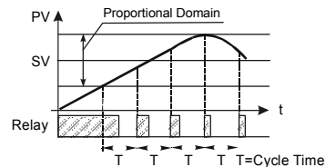
PID control with relay output
