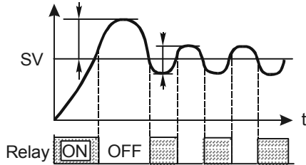
ON/OFF control without hysteresis
