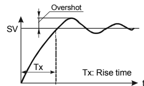
PID control with overshoot
