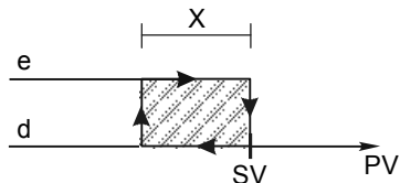
Asymmetrical hysteresis band in reverse control. (Pump-in/Filling control)
