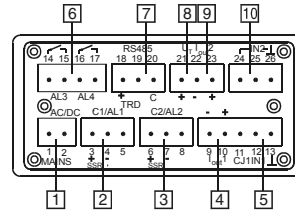
Models with SSR drive output
