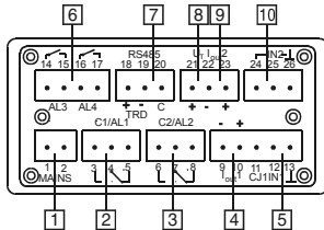
Models with relay output
